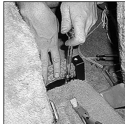
Install new bracket using 5/16" bolts, nuts and washers (Two people recommended)
