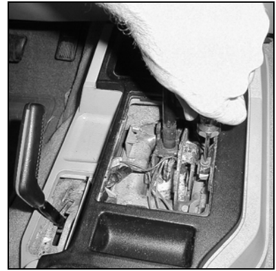
Remove screws holding black insert (see next step also).
