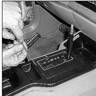
Remove transmission shift lever bezel by prying upward
