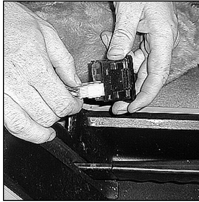
Disconnect wiring by squeezing tabs on plug
