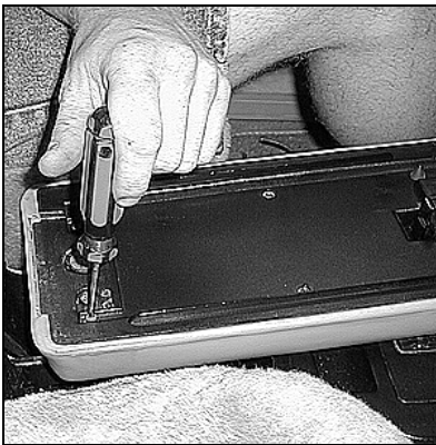
Remove screws holding plastic base on lid cushion
