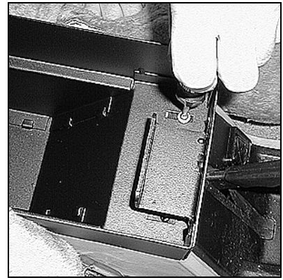
Use (2) #8x1 screws supplied to screw Tuffy console down, install the rest of the console by reversing the steps of removal
