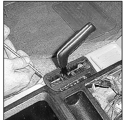
Remove transfer case shift lever bezel by prying upward
