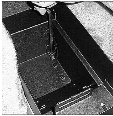
Bolt Tuffy console into place using (2)3/8"x1" bolts supplied
