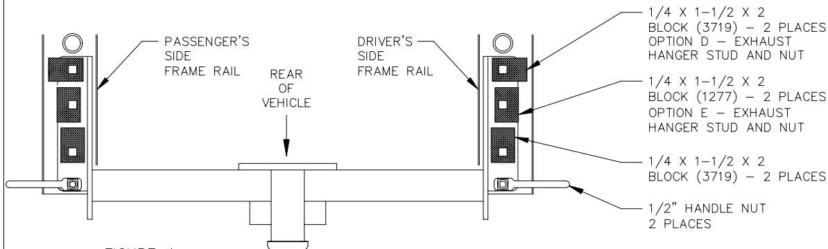
FIGURE 4 VIEWED FROM UNDER VEHICLE LOOKING UP
